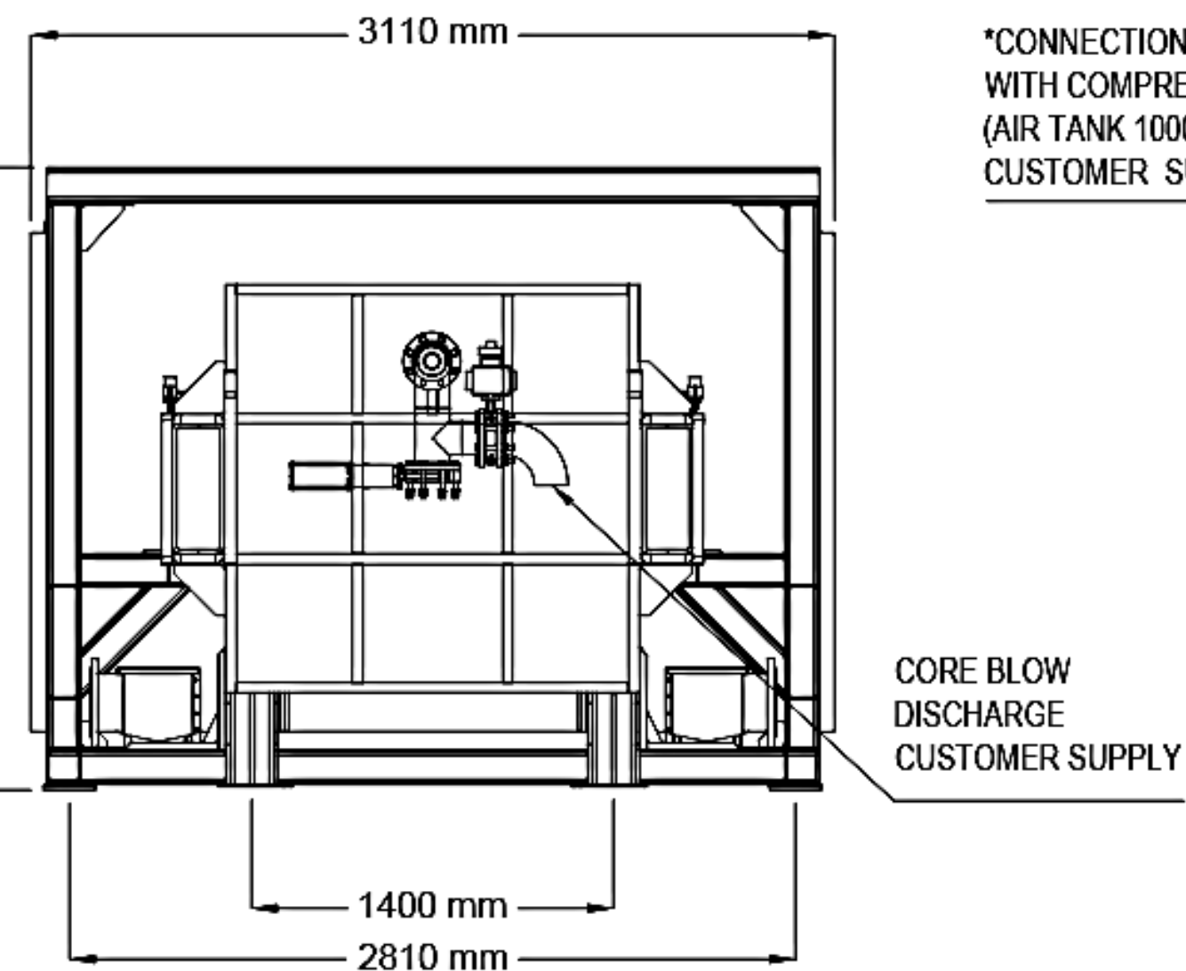
LEFT VIEW
