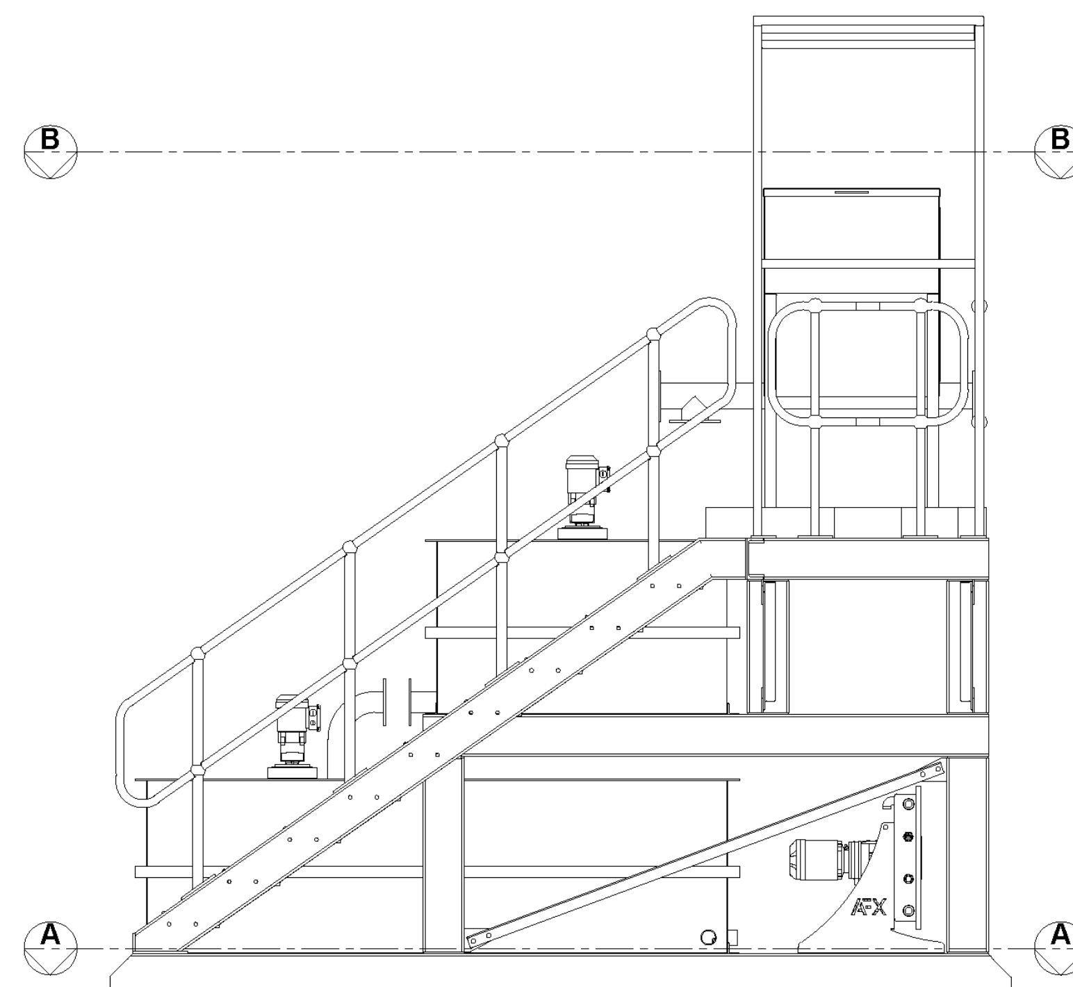
FRONT VIEW
